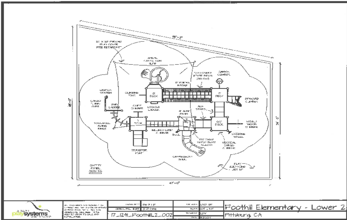
Plan of Replacement Play Structure 2 @ Foothill ES
