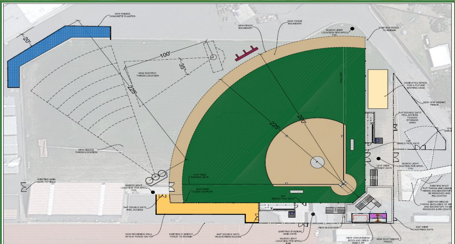
SITE PLAN - SOFT BALL FIELD SCALE : \frac{1}{16}'' = 1'-0''
