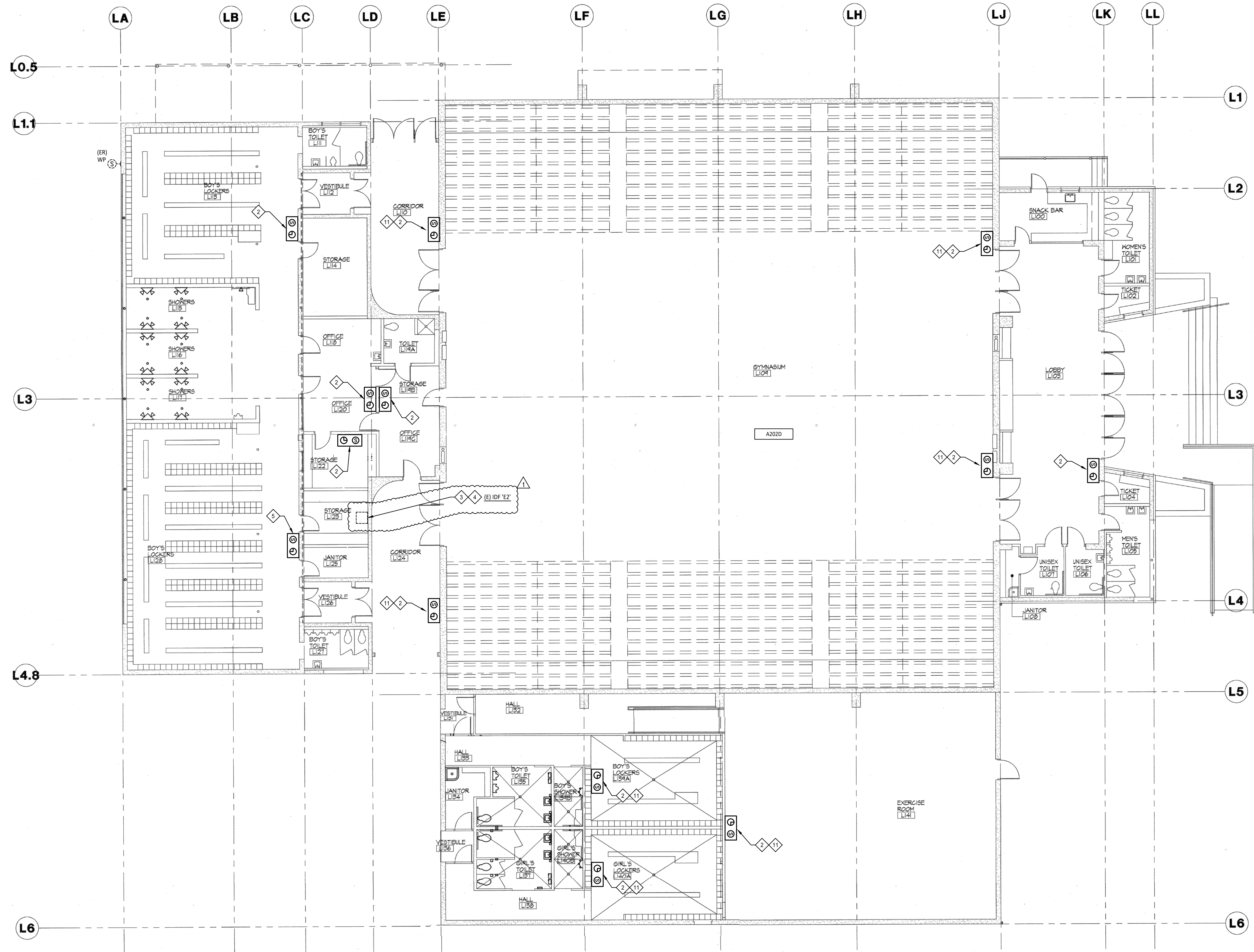
BUILDING E2 ELECTRICAL PLAN - BOYS GYMNASIUM 1/8" = 1'-0" 1
